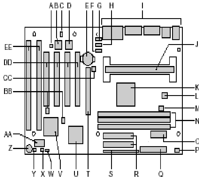
Figure 1. Motherboard Components
